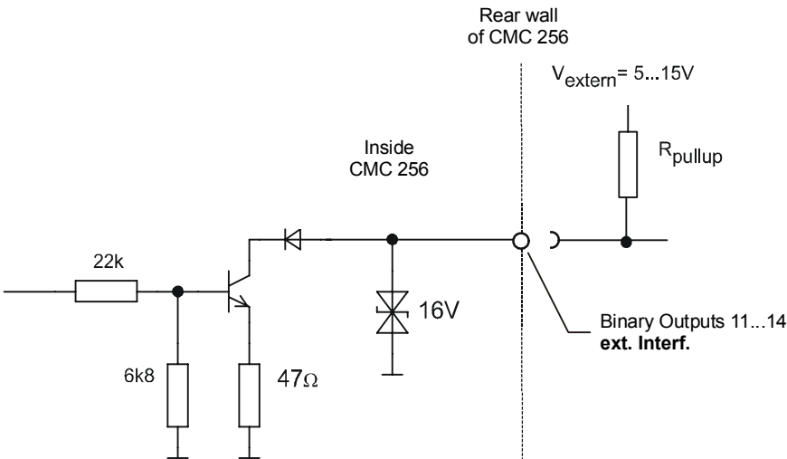
Figure 5-9: Output circuit of the binary transistor outputs 11 - 14
