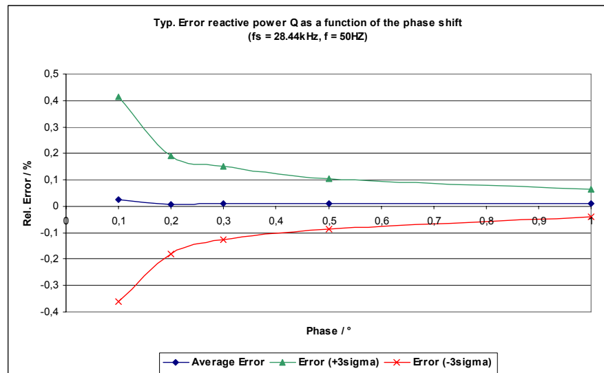
Figure 6-21: Typical error 1 of the reactive power Q as a function of the phase shift considering the apparent power, f_s=28.44\text{kHz} , f_{in}=50\text{Hz} , excitation CH1 and CH2 = 70%.
