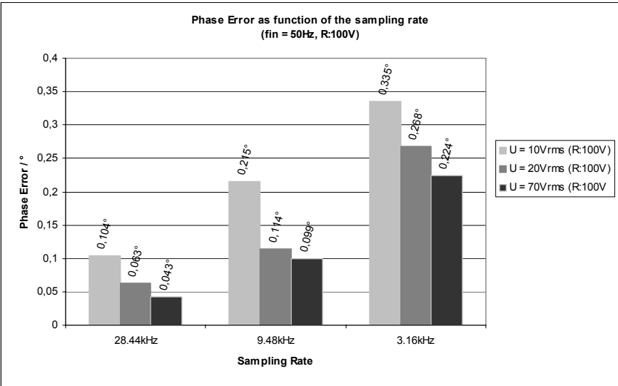
Figure 6-15: Phase error as a function of the sampling rate
