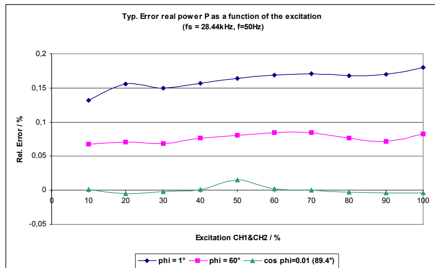
Figure 6-19: Typical error of the real power P as a function of the excitation considering the apparent power, f_s=28.44\text{kHz} , f_{in}=50\text{Hz}
