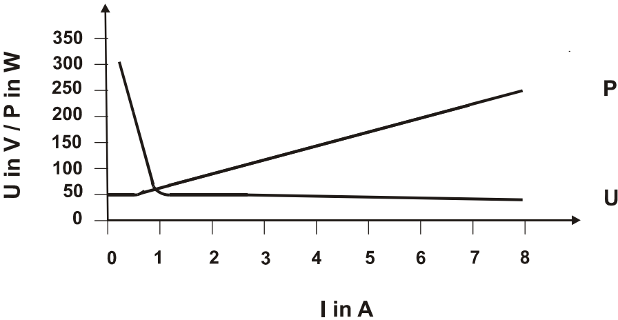
Figure 6-8: Load limit curve for relays on the binary outputs with DC voltages
