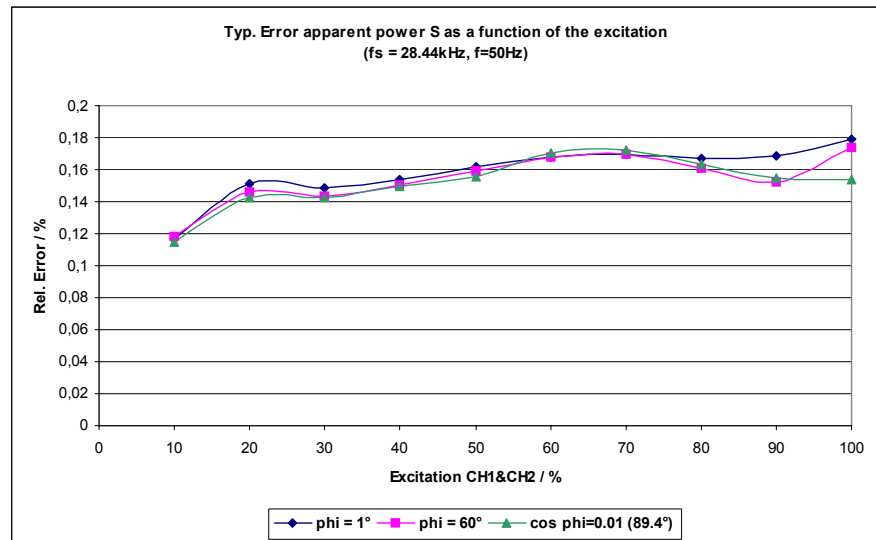
Figure 6-18: Typical error of the apparent power S as a function of the excitation, f_s=28.44\text{kHz} , f_{in}=50\text{Hz}
