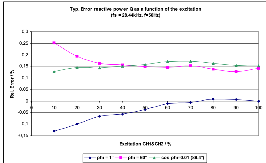
Figure 6-20: Typical error of the reactive power Q as a function of the excitation, f_s=28.44\text{kHz} , f_{in}=50\text{Hz}
